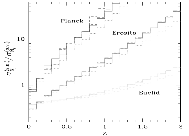
Fig. K.1. The ratio \sigma_{N_i}^{(s.n.)} / \sigma_{N_i}^{(s.v.)} of the rms shot-noise contribution \sigma_{N_i}^{(s.n.)} to the rms sample-variance contribution \sigma_{N_i}^{(s.v.)} , of the covariance of the angular number densities N_i , as in Fig. 34. The fiducial curve that was shown in Fig. 34 is the solid line (mean WMAP7 cosmology), whereas the dashed, dot-dashed, and dotted lines correspond to the three cosmologies where either h , \Omega_m , or \sigma_8 is changed to the value given in the second line of Table K.1.
