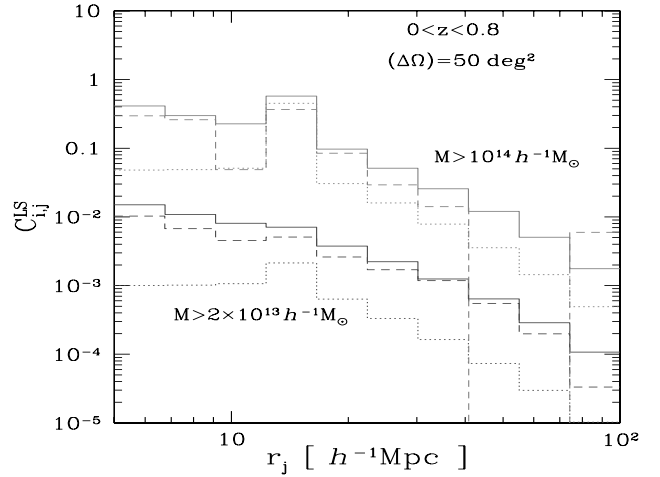
Fig. 18. The covariance matrix C_{i,j}^{\text{LS}} , as in Fig. 17, but along one row. This corresponds to the fixed bin i = 4 , associated with the distance bin 12.3 < r < 16.6 h^{-1} \text{ Mpc} , as a function of j .
