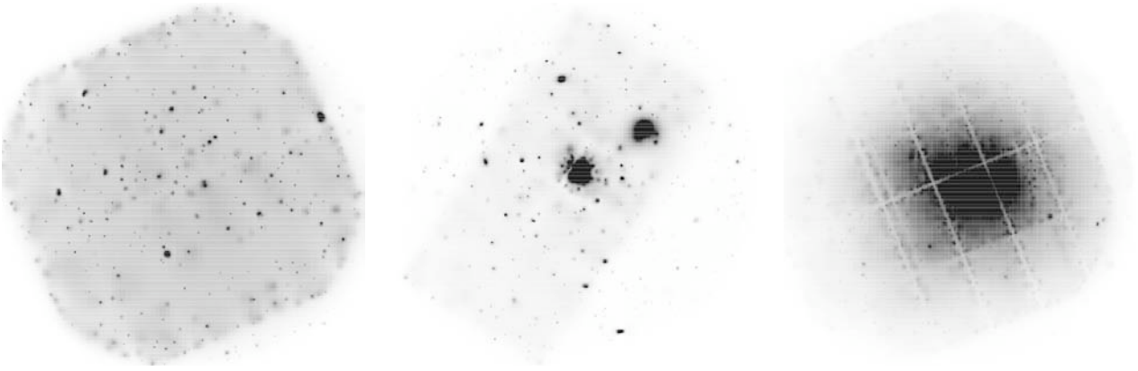
Figure 8. Three examples of pointings excluded from the cosmological analysis (images have been filtered by wavelets). Left panel: this pointing shows a high background on the PN detector which has not been optimally filtered by the pre filtering procedure due to long continuous periods of background flares (ObsId: 0039140101). Central panel: the PN detector was working in Large Window mode thus not collecting photons from the entire field of view (ObsId: 0083150401). Right panel: observation of Coma extending over a large part of the field of view thus preventing the detection of background sources (ObsId: 0300530301).
