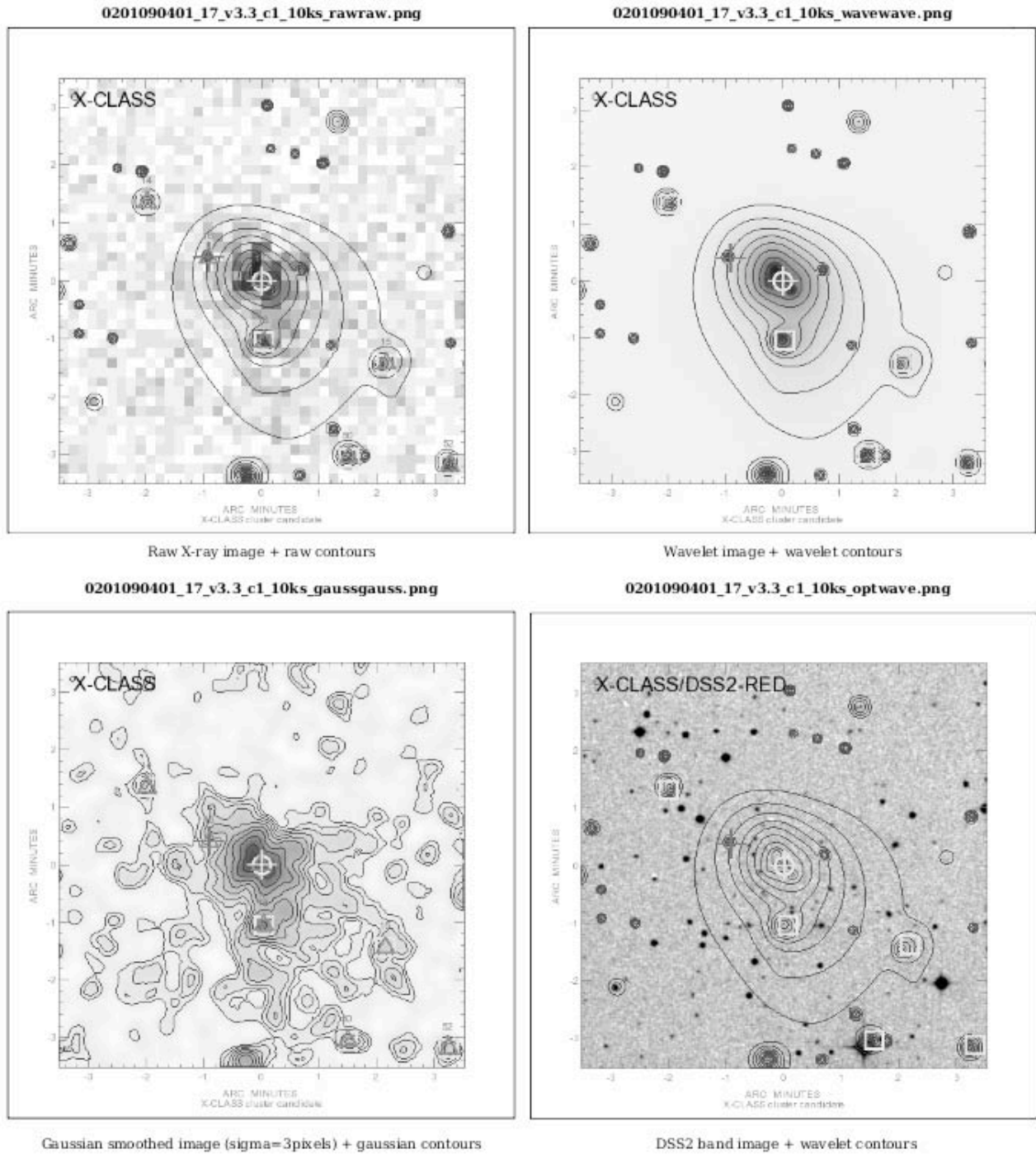
Figure A2. Screenshot of a webpage from the X-CLASS database ( http://xmm-lss.in2p3.fr:8080/14sdb/ ), for a particular cluster (tag 908). Displayed are the X-ray photon image ( top-left ) with associated contours, the wavelet-filtered ( top-right ) and gaussian-filtered ( bottom-left ) images and the optical (POSS-II) overlay ( bottom-right ).
