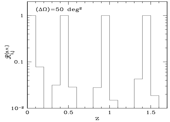
Fig. 11. The correlation matrix \mathcal{R}_{i,j}^{(s.v.)} of Eq. (46) between redshift bins of width \Delta z = 0.1 . We show \mathcal{R}_{i,j}^{(s.v.)} as a function of j , for four values of i . In each case, \mathcal{R}_{i,i}^{(s.v.)} = 1 at j = i . We consider halos above 10^{14} h^{-1} M_{\odot} and an angular window of area (\Delta\Omega) = 50 \text{ deg}^2 .
