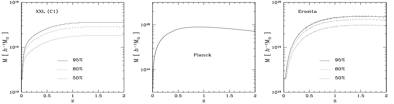
Fig. J.1. Left panel: cluster mass associated with a 50%, 80%, or 95% detection probability (from bottom to top), for the XXL selection function C1, as a function of redshift. Middle panel: minimum detectable cluster mass, as a function of redshift, for the Planck space mission. Right panel: cluster mass associated with a 50%, 80%, or 95% detection probability (from bottom to top), for the Erosita selection function as a function of redshift (we consider a flux limit of 4 \times 10^{-14} erg s ^{-1} cm ^{-2} in the [0.5–2] keV band).
